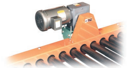
OPTIONAL TOP ROLLER GUARD MOUNTED DRIVE
